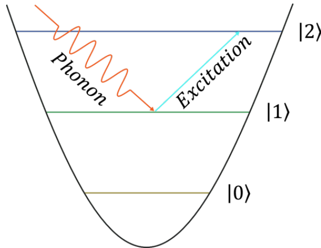
Figure 1: Phonon Stimulated Excitations
