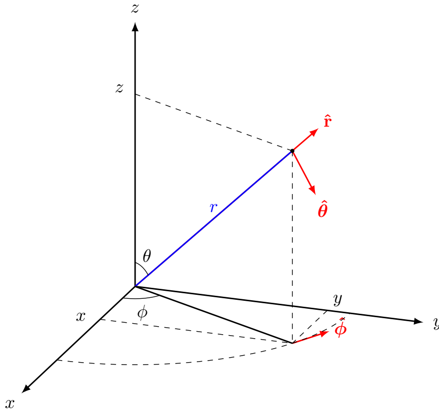
Figure 1: The spherical coordinates.
