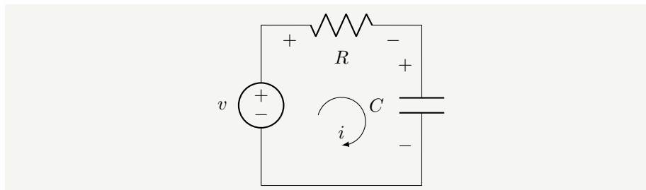
Figure 8: Converting Pulse Width Modulated (PWM) signal to its DC value. The capacitor charges to the mean value of the PWM. For 255 this will be the half of the supply voltage, i.e., will yield 2.5V.
